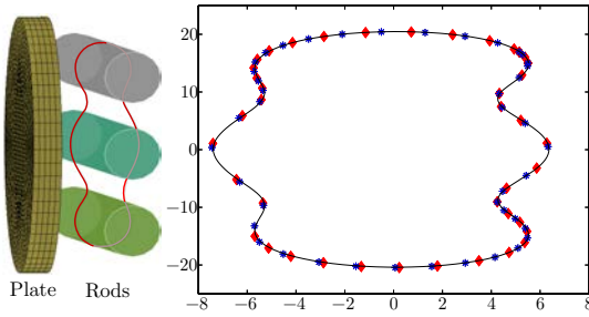
Figure 2: Direct method: —, multipole method: \blacklozenge , multicenter method: *
