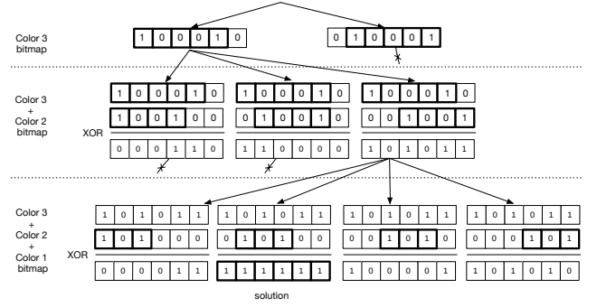
Figure 3. Bitmap evaluation of color alignments.
