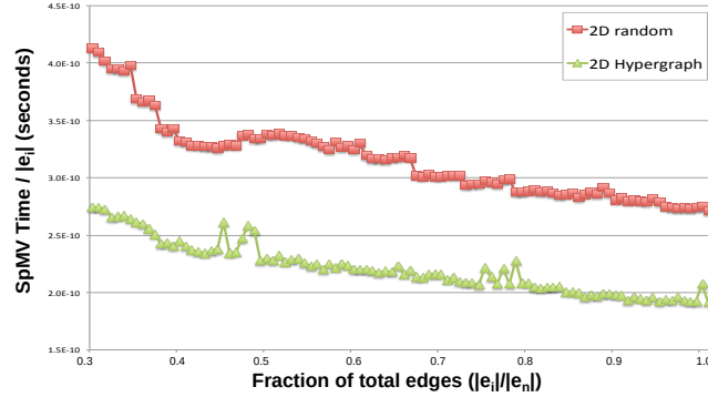
Figure 2: SpMV time in seconds (normalized by number of nonzeros) as graph evolves.
