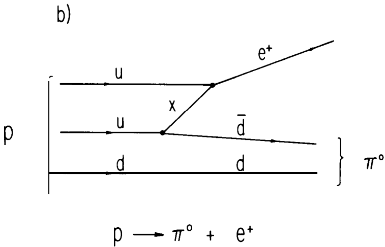
Fig. 6. (a) Simplified diagrams of baryon number non-conserving X boson decays. (h) A proton decay mediated by an X boson.
