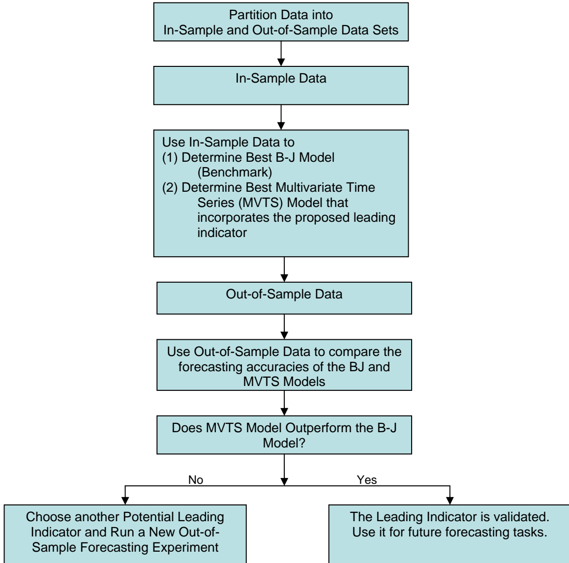
Figure 3 Out-of-Sample Forecasting Experiments: Validating Proposed Leading Indicators
