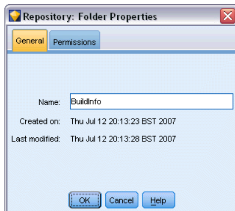
Figure 9-18 Folder properties
