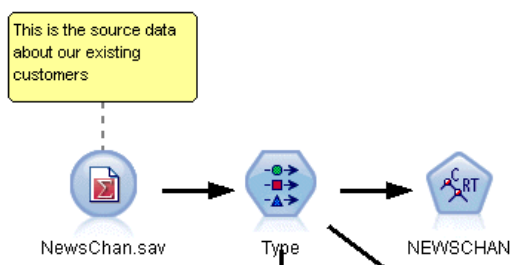
Figure 5-33 Completed comment
