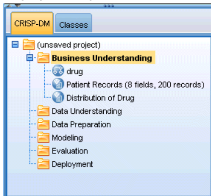
Figure 3-10 CRISP-DM view
