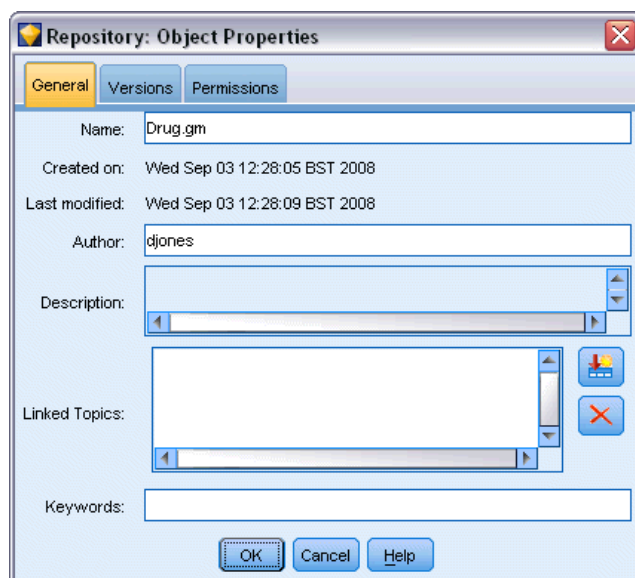
Figure 9-20 Object properties
