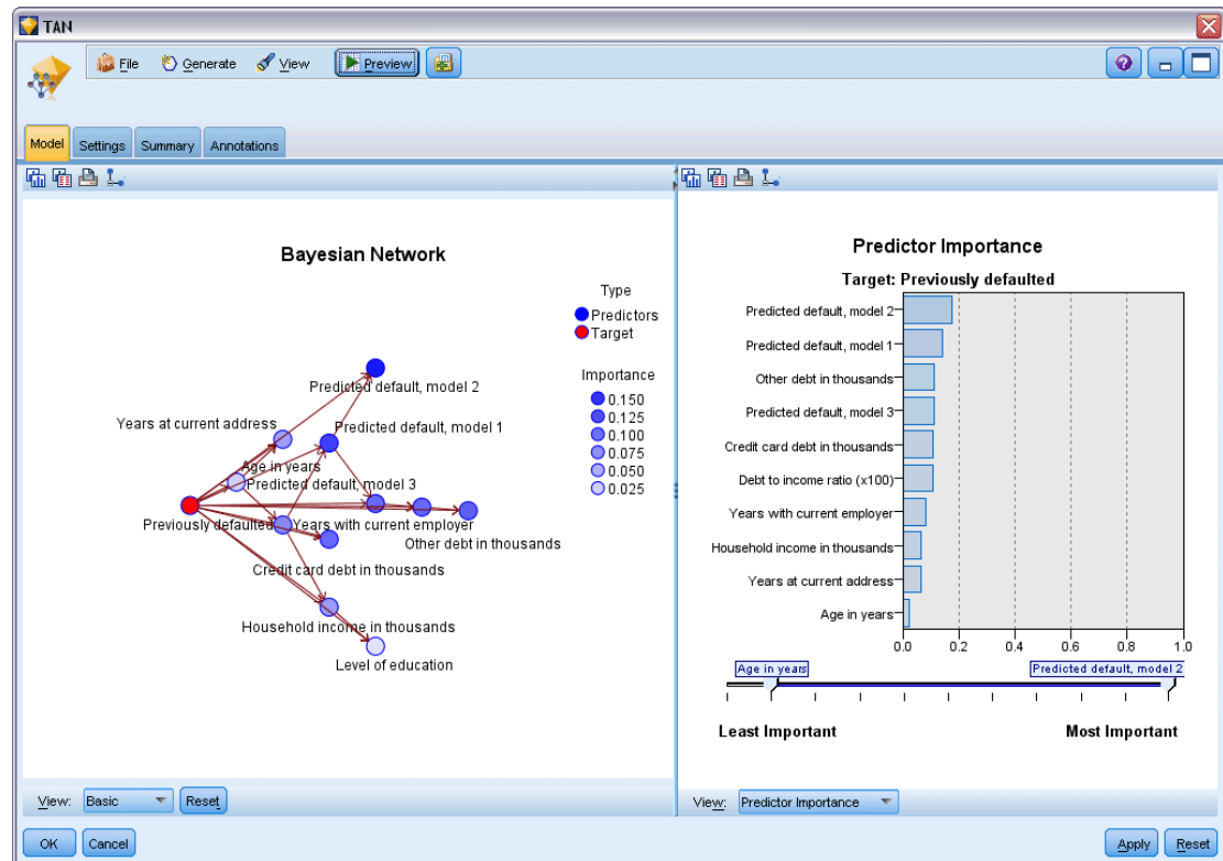
Figure 18-7 Viewing a Tree Augmented Naïve Bayes model
