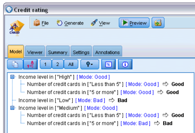
Figure 4-9 CHAID model nugget, rule set
