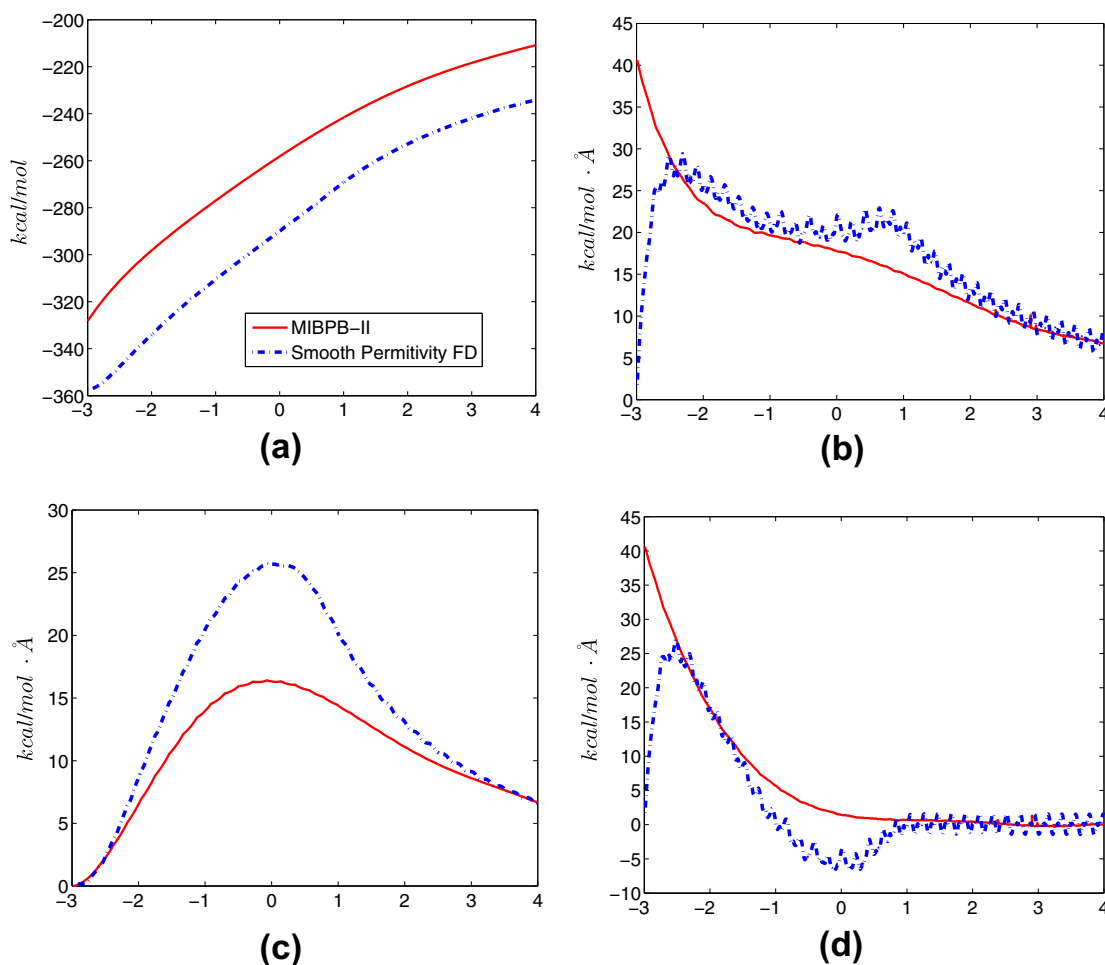
Fig. 5. Comparison of electrostatic forces on the moving atom of a two-atom systems obtained at h = 0.21 \text{ \AA} . The horizontal axis is the position of the moving atom in unit \text{\AA} . Red solid line: present MIB based method with molecular surfaces; Blue dotted line: PBEQ with smooth interface: (a) solvation free energy of the system, (b) total force on the moving atom calculated from the summation of reaction force and dielectric boundary force, (c) reaction force, (d) dielectric boundary forces. (For interpretation of the references to colour in this figure legend, the reader is referred to the web version of this article.)
