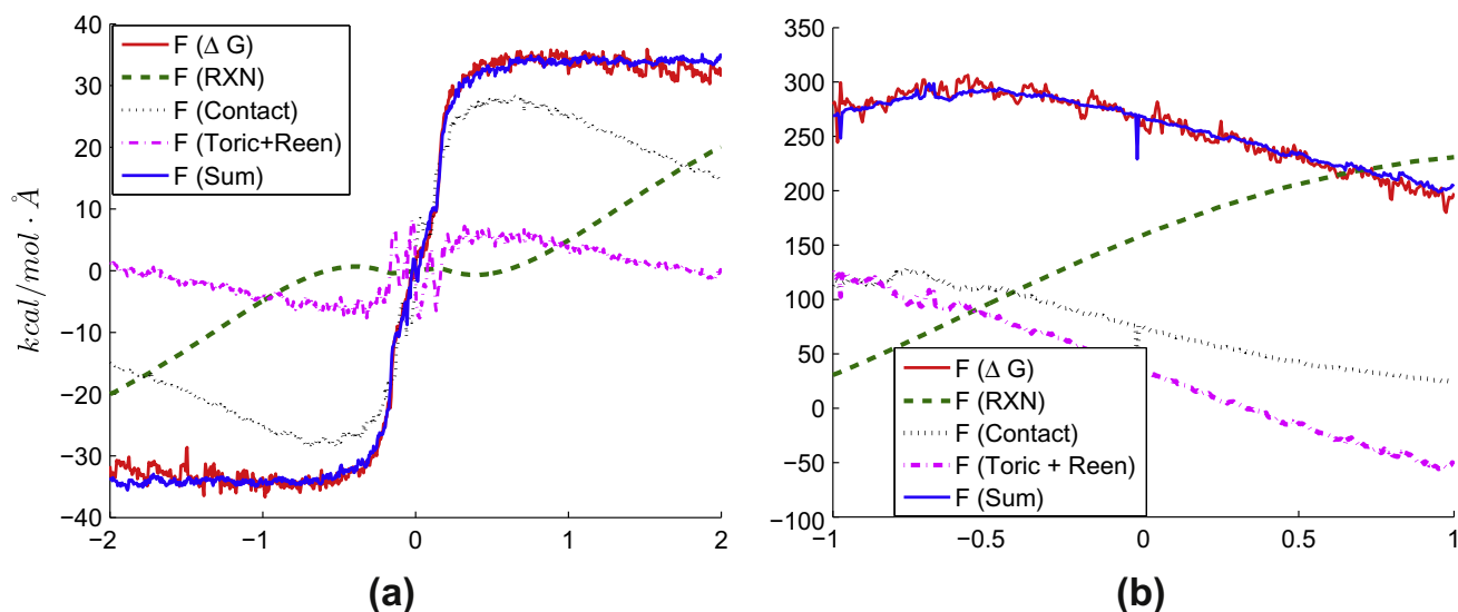
Fig. 6. Forces calculated for (a) a three-atom system and (b) Cyclohexane. The horizontal axis is the position of the moving atom in unit Å and the vertical axis is the forces.
