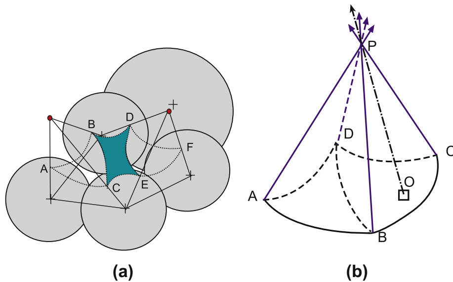
Fig. 2. Dielectric boundary force calculation: (a) illustration of reentrant surfaces, e.g. ABC and DEF , and toric surfaces, e.g. CEDB in green, on the molecular surface; (b) force distribution from a reentrant surface to related atoms.
