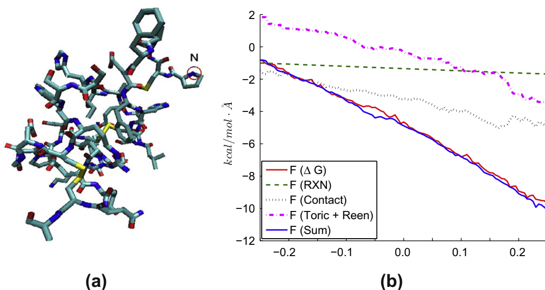
Fig. 7. A low-density lipoprotein receptor 1ajj: (a) Illustration of the molecule and the atom that is moved, (b) Electrostatic forces. The horizontal axis is the position of the moving atom in unit Å and the vertical axis is the forces.
