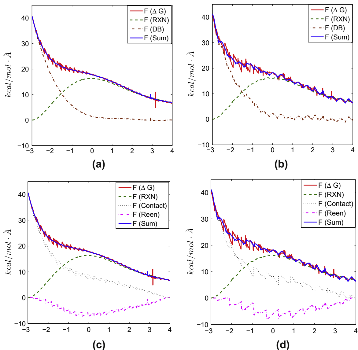
Fig. 4. Electrostatic forces calculated for two separating charged atoms. The horizontal axis is the position of the moving atom in unit Å and the vertical axis is the forces: (a) h = 0.21 Å with summed dielectric boundary forces, (b) h = 0.42 Å with summed dielectric boundary forces, (c) h = 0.21 Å with decomposed dielectric boundary forces, (d) h = 0.42 Å with decomposed dielectric boundary forces.
