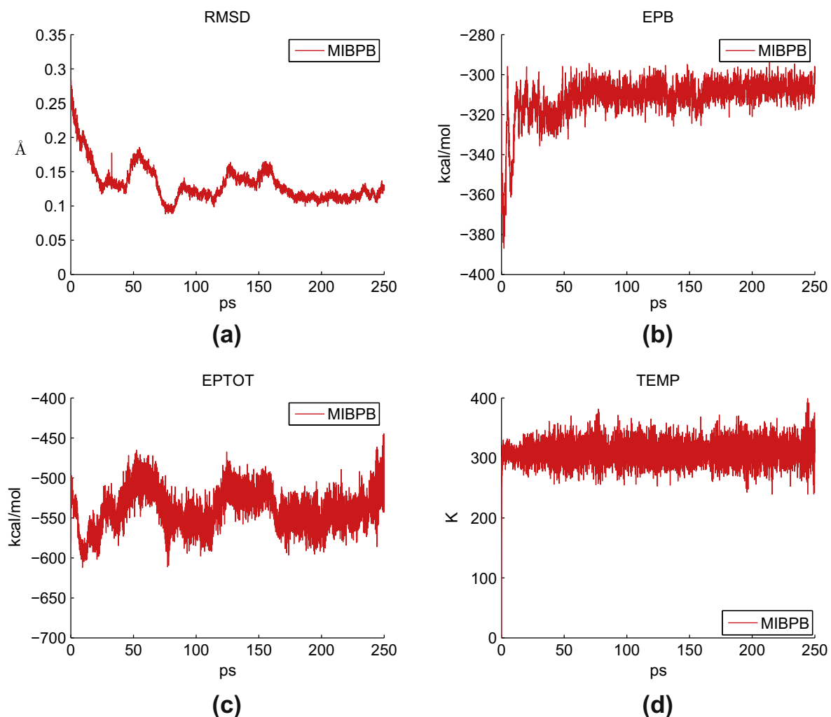
Fig. 12. 250 ps MD simulations of the Trp-cage mini-protein (1L2Y) obtained with the MIBPB method. The horizontal axis is time in unit of picosecond (ps): (a) RMSD, (b) solvation free energy, (c) total potential energy, (d) temperature.
