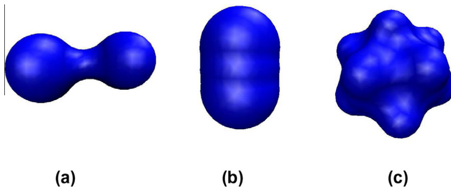
Fig. 3. Molecular Surface generated from MSMS for (a) a diatomic system, (b) a three-atom system, and (c) Cyclohexane (18 atoms).
