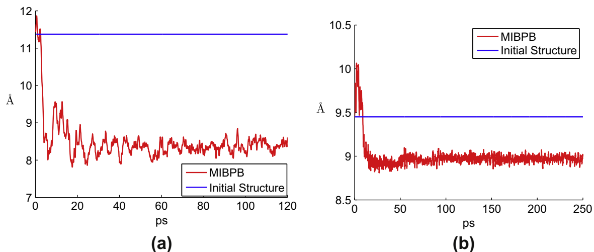
Fig. 11. A comparison of the averaged C_{\alpha} atom distances. The horizontal axis is time in unit of picosecond (ps) and the vertical axis is distance. The red line is the simulation result and the blue line is that from NMR data. Results of the MIBPB are illustrated in red lines: (a) the averaged C_{\alpha} atom distances for WW domain binding protein-1 (Case 2), (b) the averaged C_{\alpha} atom distances for Trp-cage mini-protein (Case 3).
