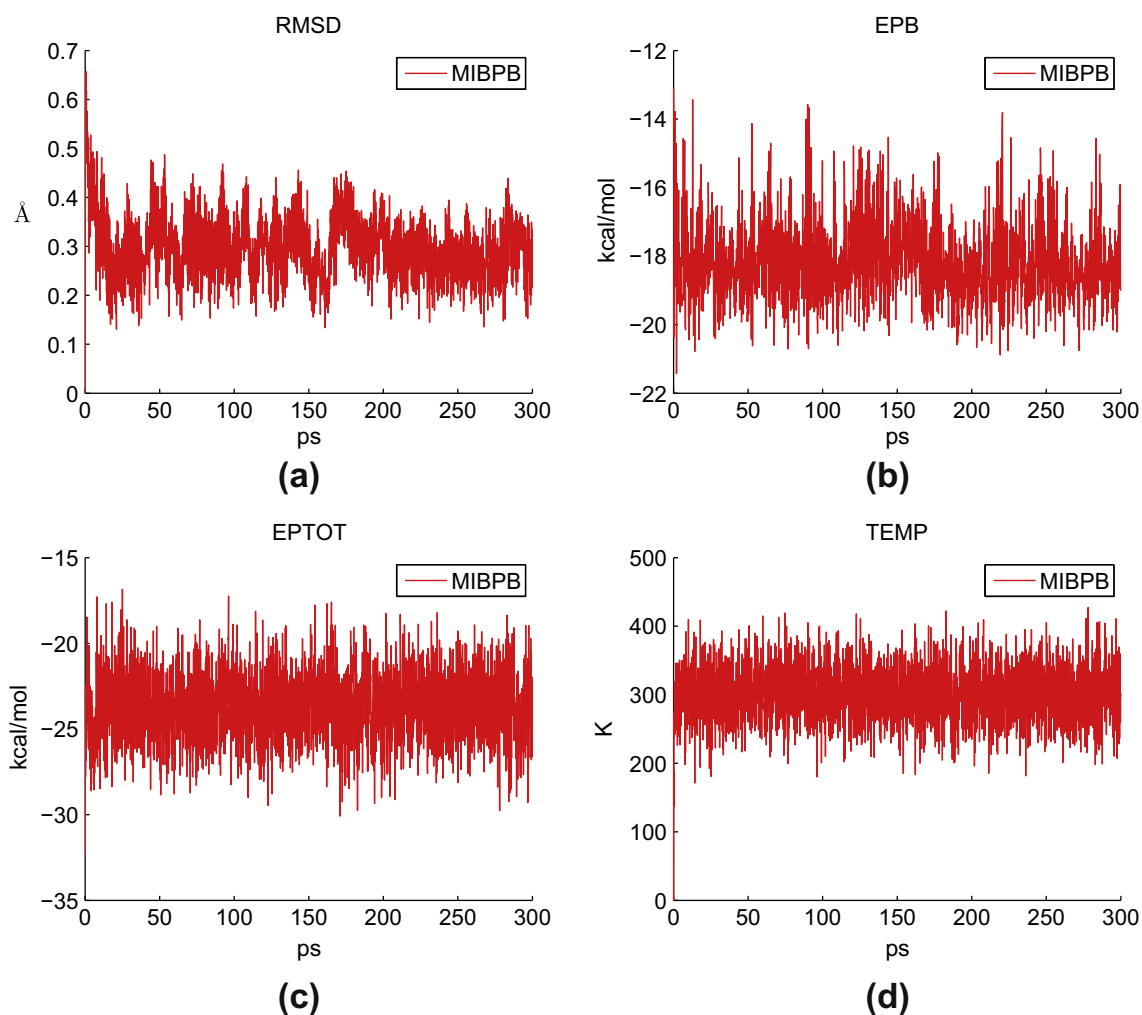
Fig. 9. 300 ps MD simulations of the alanine dipeptide obtained with MIBPB based methods. The horizontal axis is time in unit of picosecond (ps): (a) RMSD, (b) solvation free energies, (c) total potential energies, (d) temperature.
