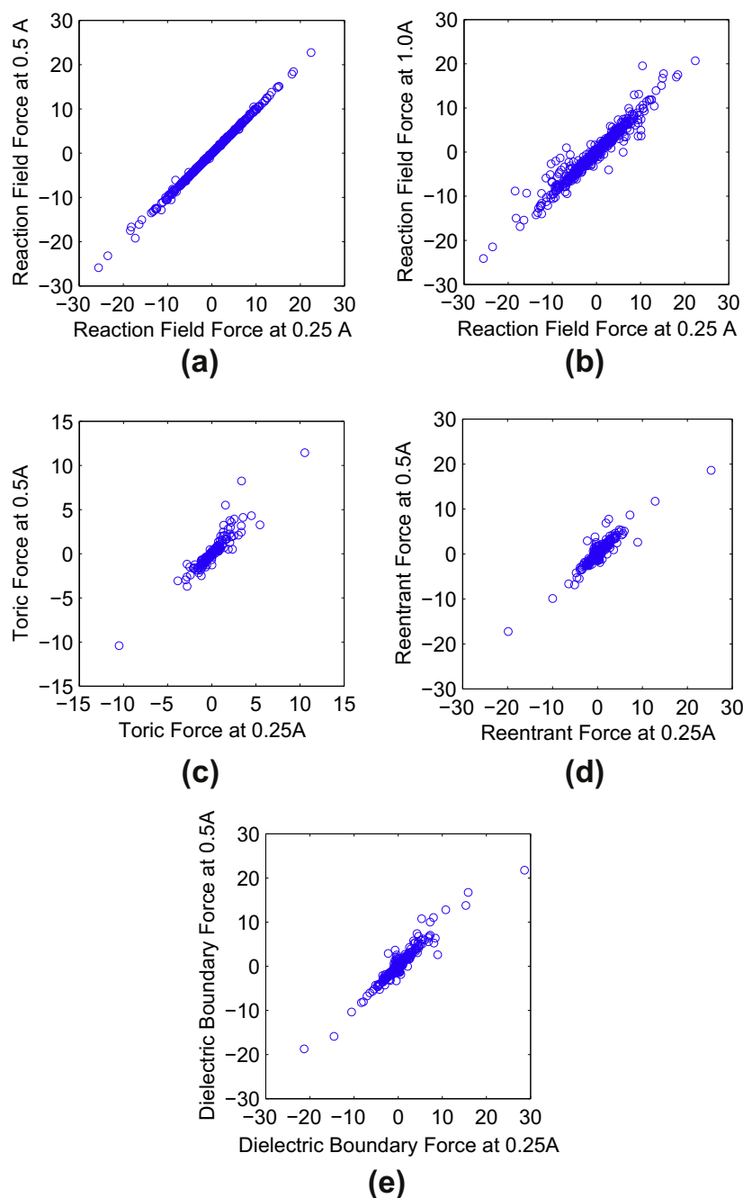
Fig. 8. Correlations of forces obtained at different mesh sizes by the MIBPB for protein 1ajj: (a) reaction field forces between mesh sizes of 0.25 and 0.5 Å, (b) reaction field forces between mesh sizes of 0.25 and 1.0 Å, (c) toric forces between mesh sizes of 0.25 and 0.5 Å, (d) reentrant forces between mesh sizes of 0.25 and 0.5 Å, (e) dielectric boundary forces between mesh sizes of 0.25 and 0.5 Å.
