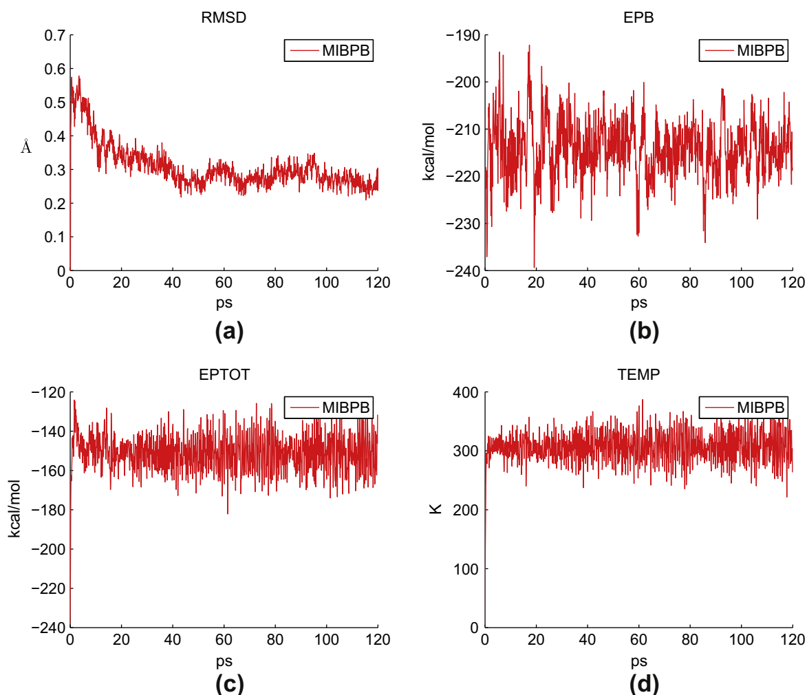
Fig. 10. A 120 ps MD simulation of the WW domain binding protein-1 obtained with the MIBPB based PB method. The horizontal axis is time in unit of picosecond (ps): (a) RMSD, (b) solvation free energy, (c) total potential energy, (d) temperature.
