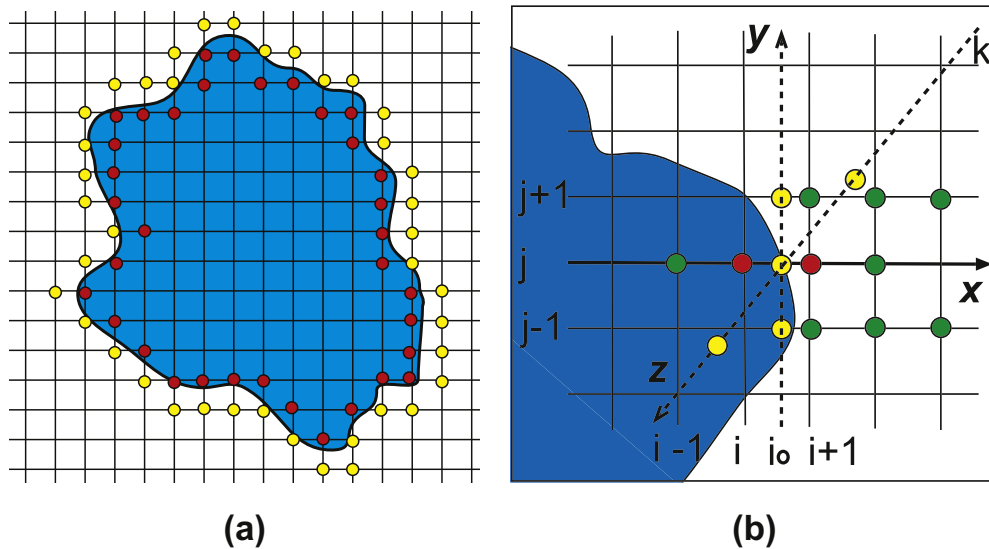
Fig. 1. An illustration of MIB schemes. The horizontal and vertical axes are the x and y directions, respectively. (a) The grid extension near the interface in a second order scheme, (b) an intersecting point at (i_0, j, k) .
