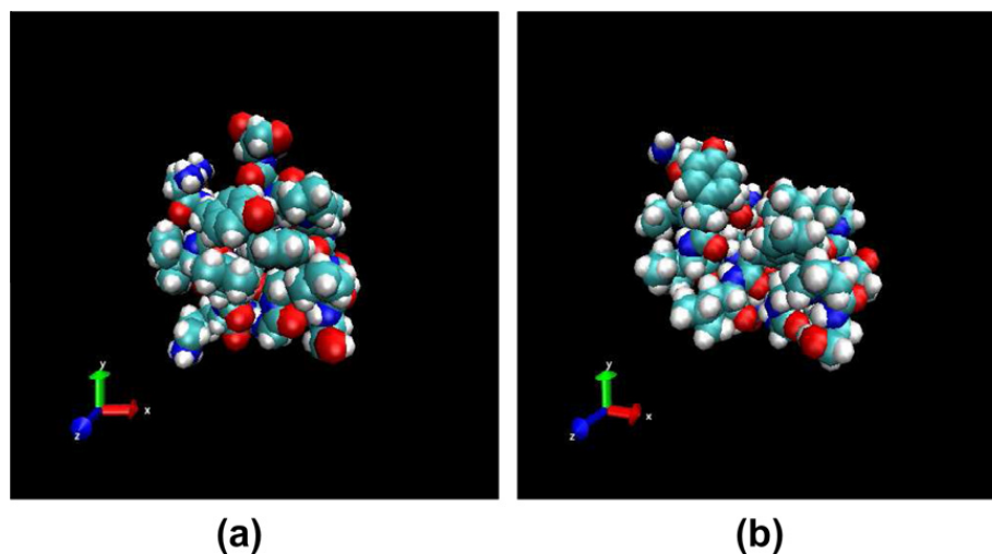
Fig. 13. A comparison of typical Trp-cage miniprotein structures obtained from NMR experiments and from MIBPB MD simulations: (a) obtained from NMR experiments as the initialization structure, (b) obtained from the MIBPB based MD simulation as the final structure.
