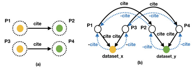
Fig. 3. Motivating Example #2
