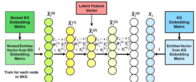
Fig. 5. One iteration of model training
