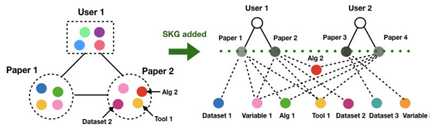
Fig. 2. Motivating Example #1
