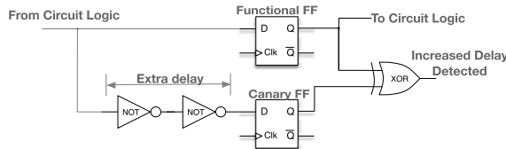
Fig. 1. Canary flip-flop design previously proposed to detect increasing delay or increase performance
