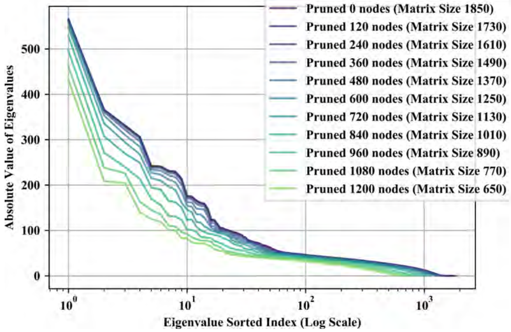
Fig. 9: Log-scaled eigenvalue index for CG spectra across different pruning levels, showing the effect of pruning on reducing low-magnitude and zero eigenvalues. The spectral information of higher-magnitude eigenvalues is preserved while the graph size decreases
