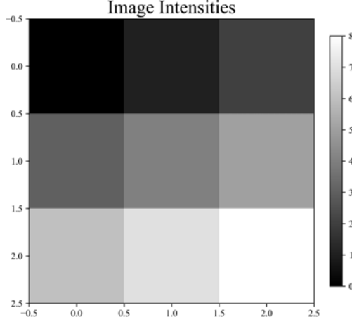
Fig. 3: Small 3 by 3 image for testing
