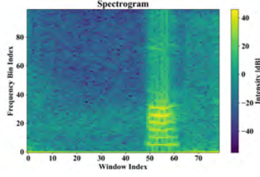
(a) DFT spectrogram for sound sample
