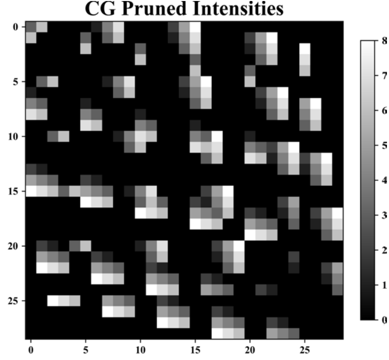
Fig. 5: Pruned Cayley adjacency
