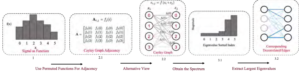
Fig. 1: Process of Cayley graph decorrelation illustrated through steps: (1) signal representation as a function, (2.1) construction of the Cayley graph adjacency matrix using permuted functions, (2.2) visualization of the Cayley graph structure, (3.1) extraction of eigenvalues sorted by magnitude, and (3.2) identification of decorrelated edges based on the largest eigenvalues.
