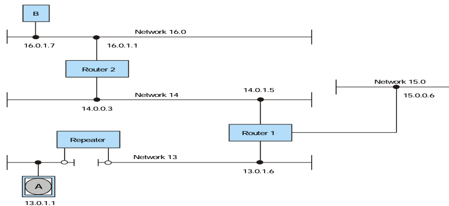
Figure 5.17 Router applications
