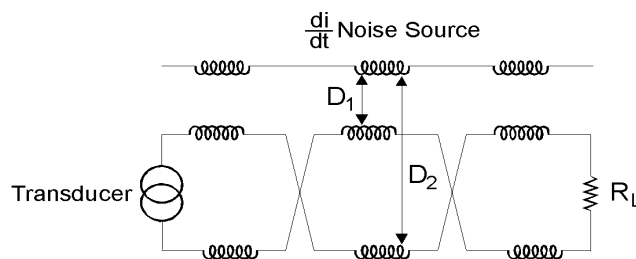
Figure 4.6 Reducing magnetic noise by twisting of wires
