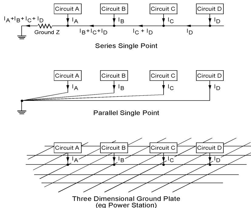
Figure 4.14 Various earthing configurations
