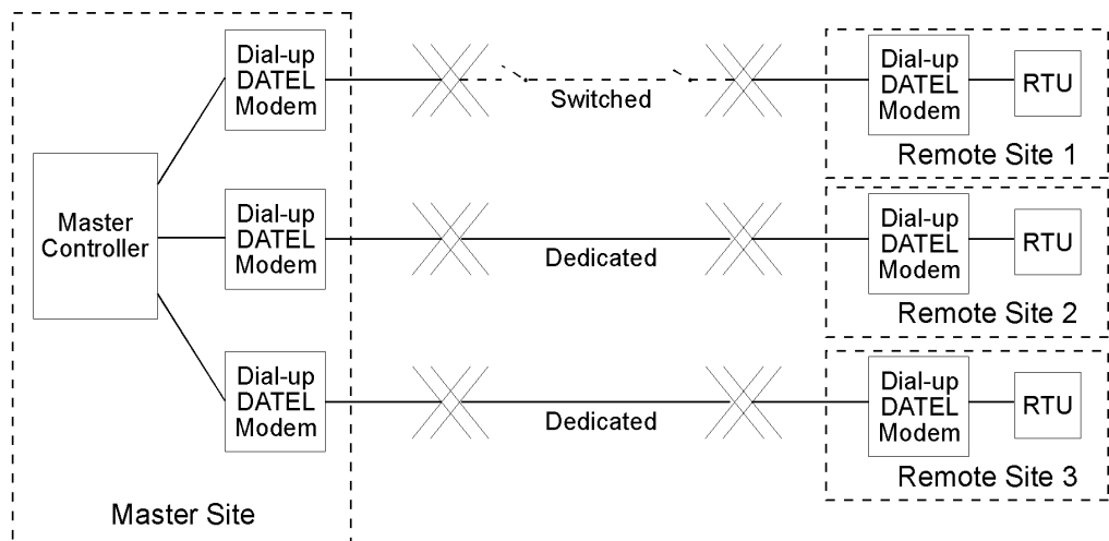
Figure 4.26 DATTEL point-to-point configuration
