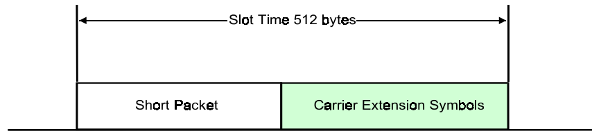
Figure 5.13 Carrier extension
