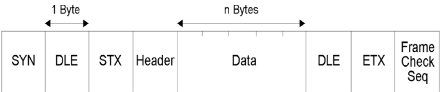
Asynchronous Data Frame
