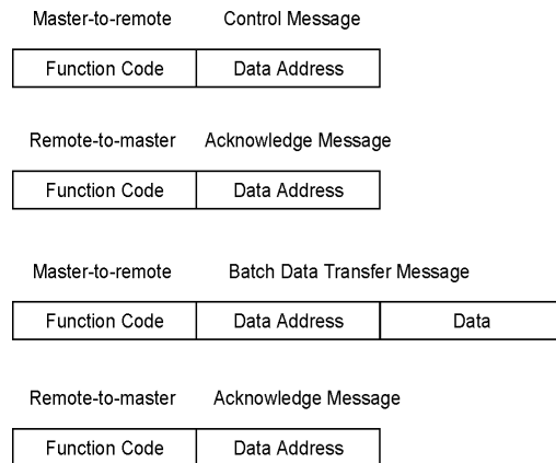
Figure 3.11 Sequence of messages for batch data transfers
