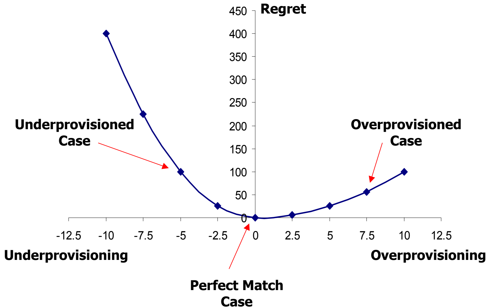
Figure 3. The Regret Function
