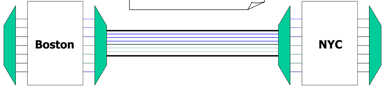
Figure 2. The Possible Cases
